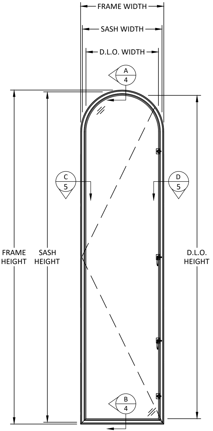
TYPICAL ELEVATION ROUND TOP
