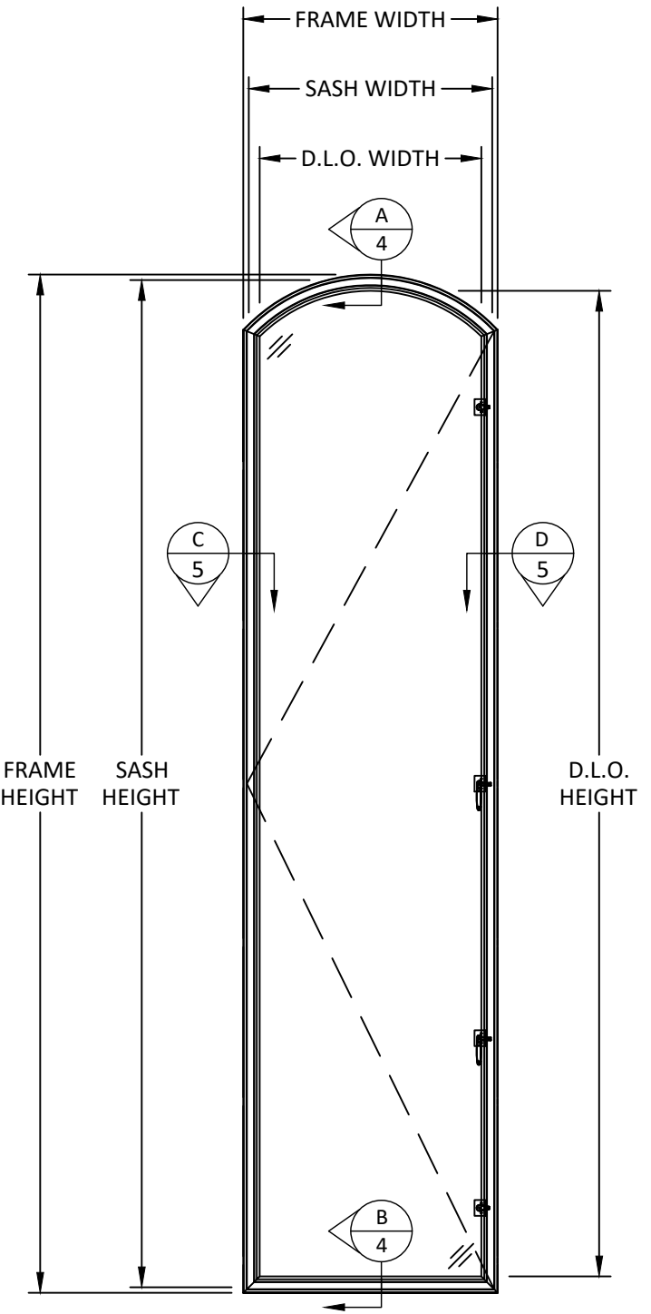
TYPICAL ELEVATION ARCH TOP
